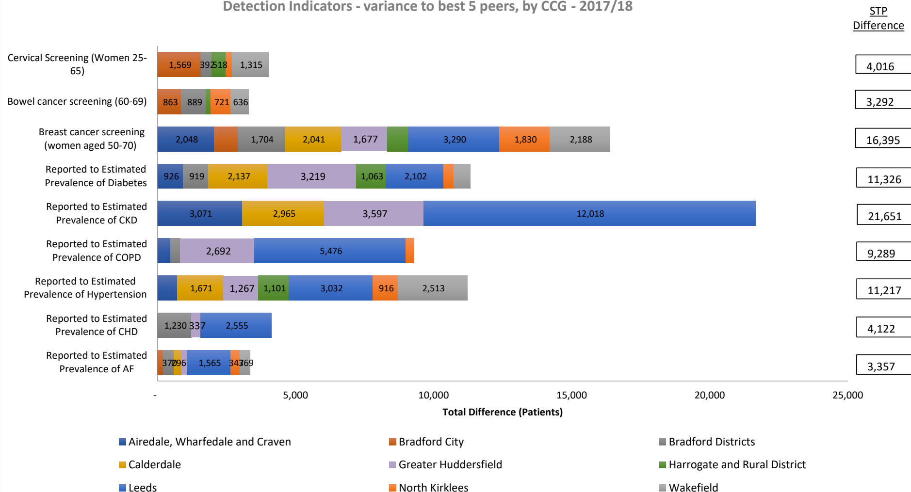
Detection Indicators - variance to best 5 peers, by CCG - 2017/18
