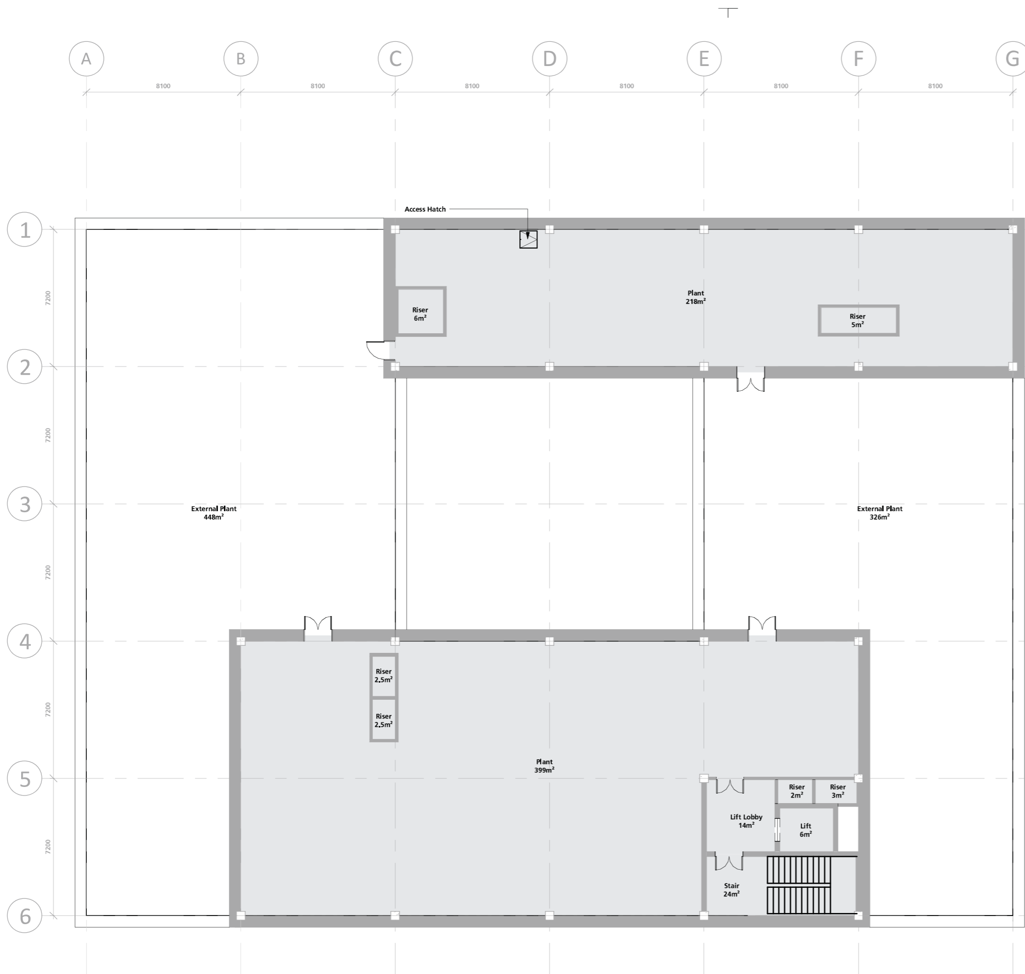
Neighbourhood health centre: core + Illustrative roof plan
