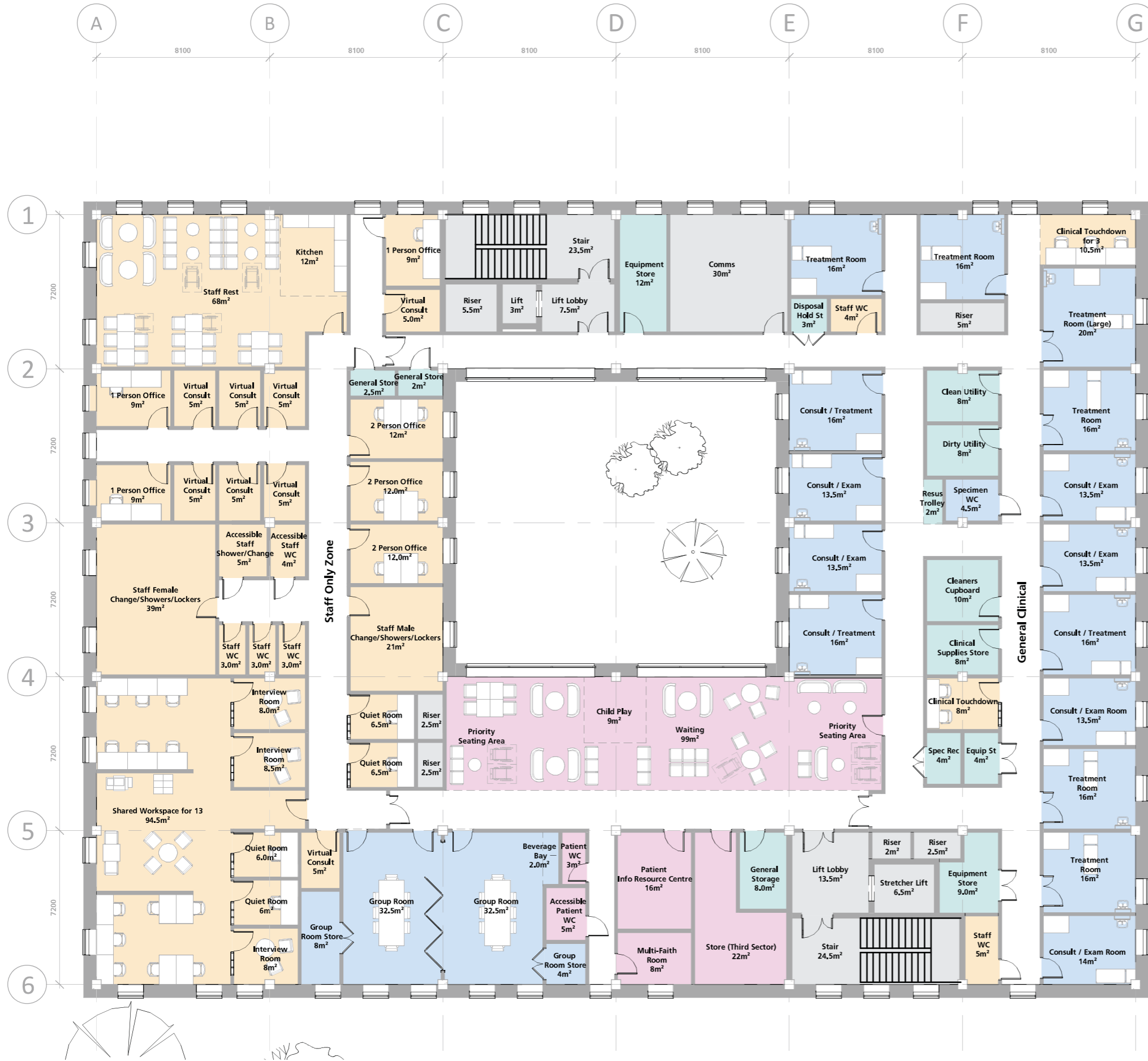
Neighbourhood health centre: core + Illustrative first floor
